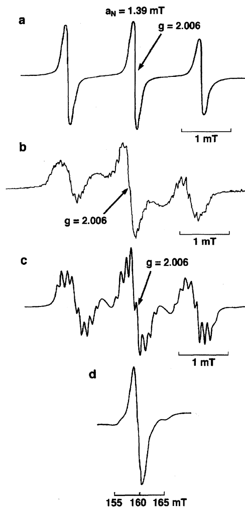
Fig. 2. ESR spectra of the polyradicals. (a) p -2 in benzene: polymer concn 1 unit mM (spin concn 0.01 spin/unit), (b) o -2 in THF: polymer concn 1 unit mM (spin concn 0.25 spin/unit), (c) 7c in THF at 1 mM, (d) o -2 in 2-methyltetrahydrofuran (spin concn 0.38 spin/unit) at 5.5 K.
